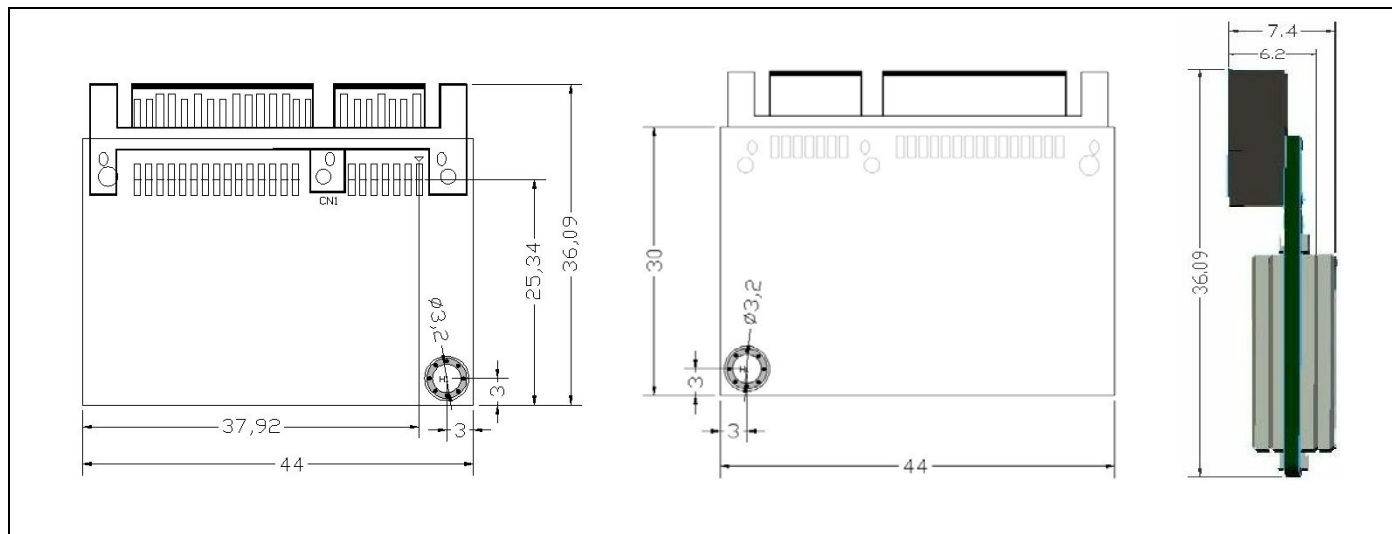
Figure 2: 7+15Pin Vertical SATA DOM Dimensions
