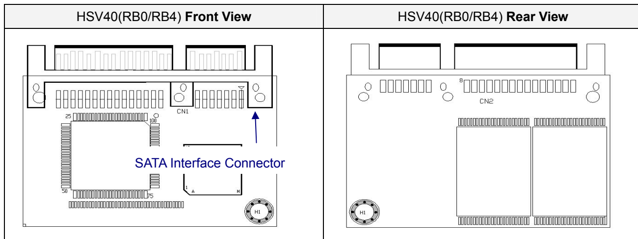
Figure 1: 7+15Pin Vertical SATA DiskOnModule Overlook Diagram
