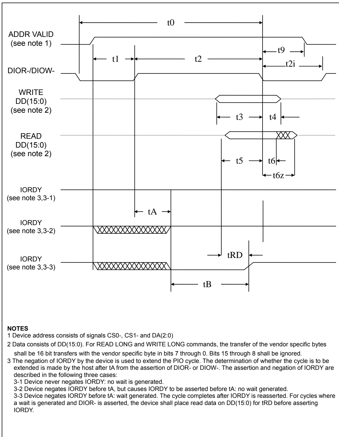
Figure 7 : PIO data transfer to/from device
