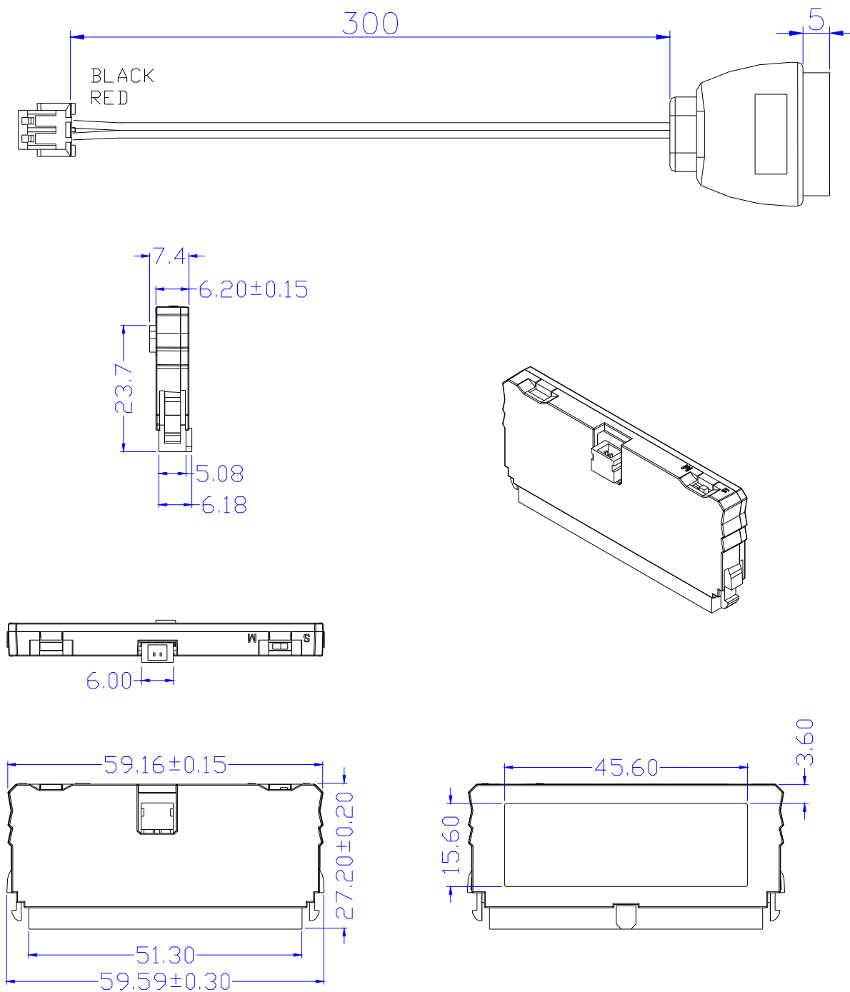
Figure 2: DOM Dimensions
